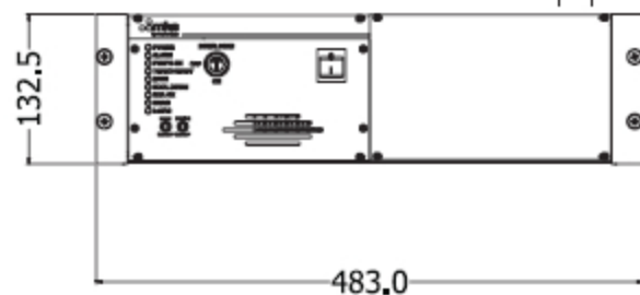
FRONT VIEW ON RVC/DSU/SUBRACK
